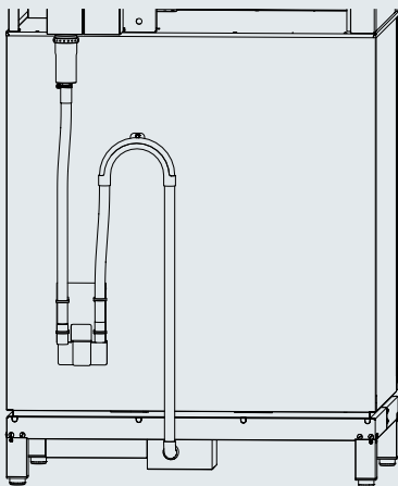
Drain lift system on a Stackit oven
